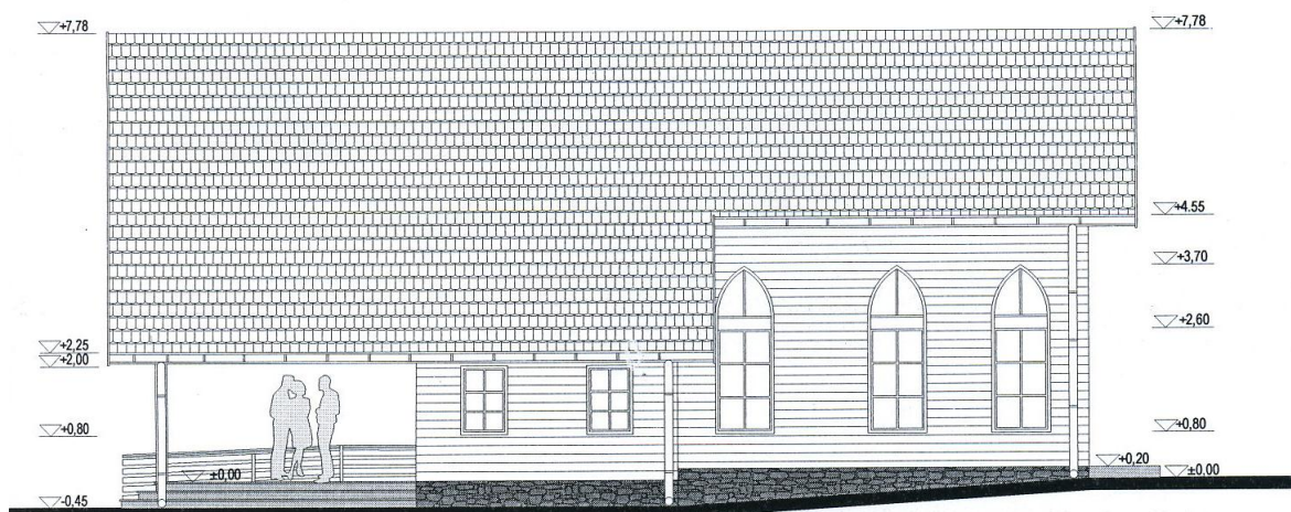
FATADA LATERALA DREAPTA ± 0.00 SC 1:100
